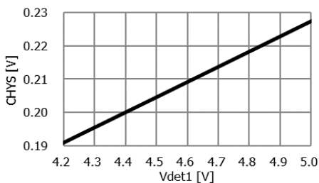
fig1. Overcharge hysteresis
